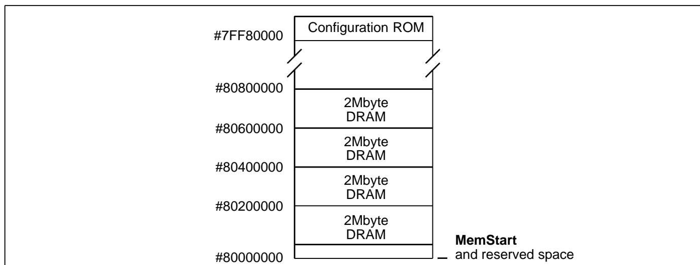
Figure 1.2 IMS B927 memory map
