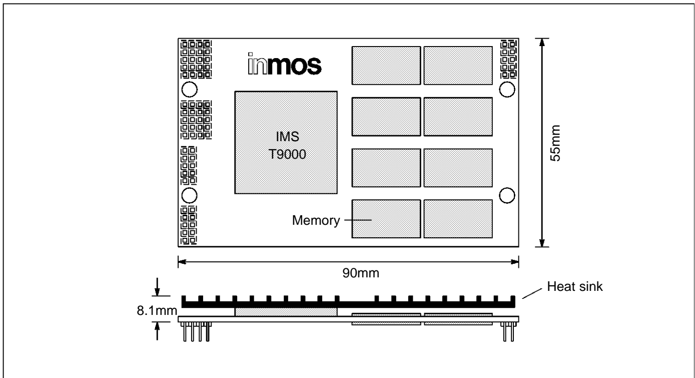
Figure 1.1 IMS B927 dimensions
